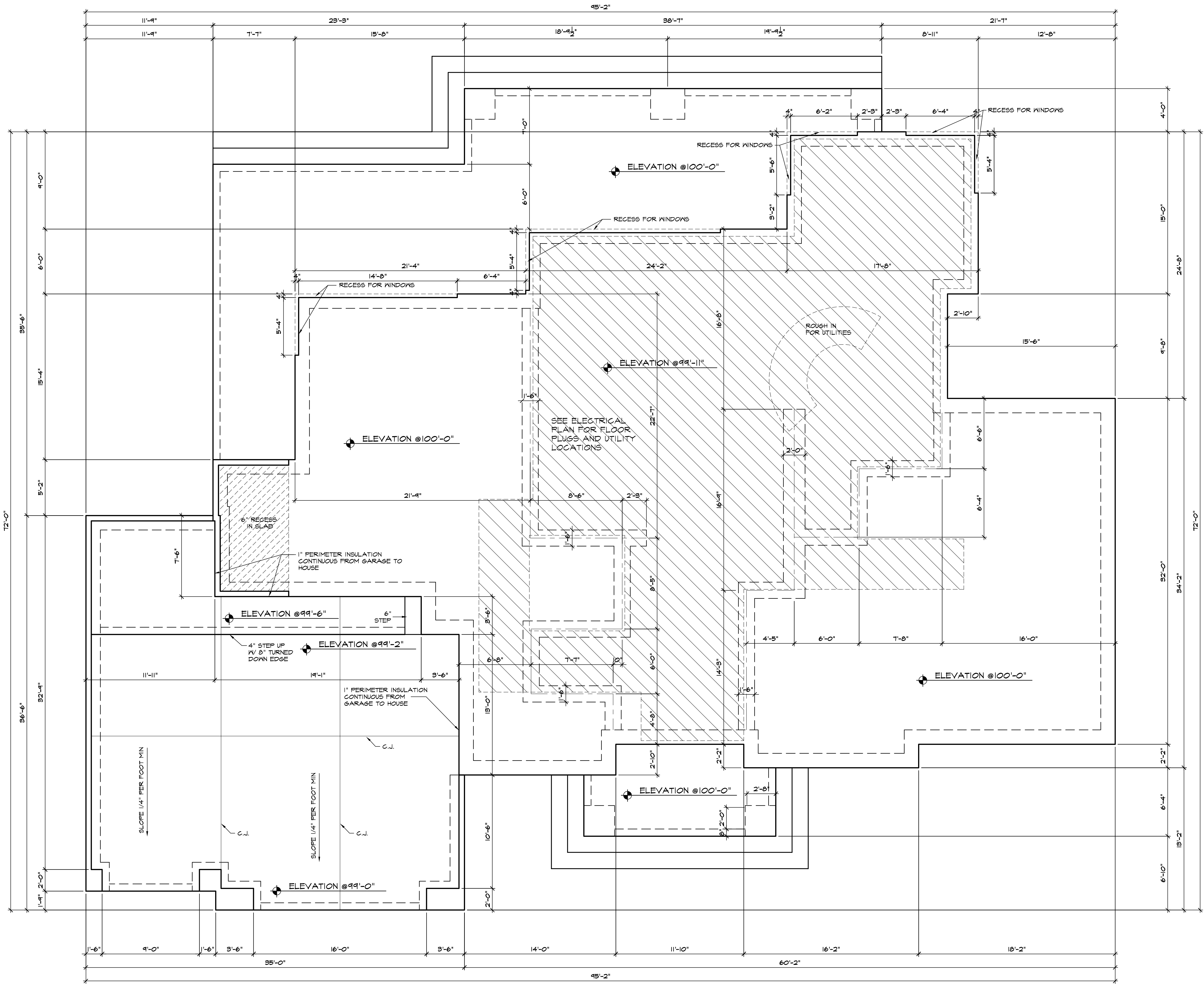
FOUNDATION PLAN
